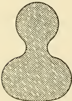
Fig. 180. Section of a "Figure 8" Trolley Wire
